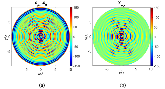
Fig. 1. Modulated sheet transition IBC for a MTS radiating a “fish like” beam a) X_{\rho\rho} - X_0 and b) X_{\rho\phi} .
