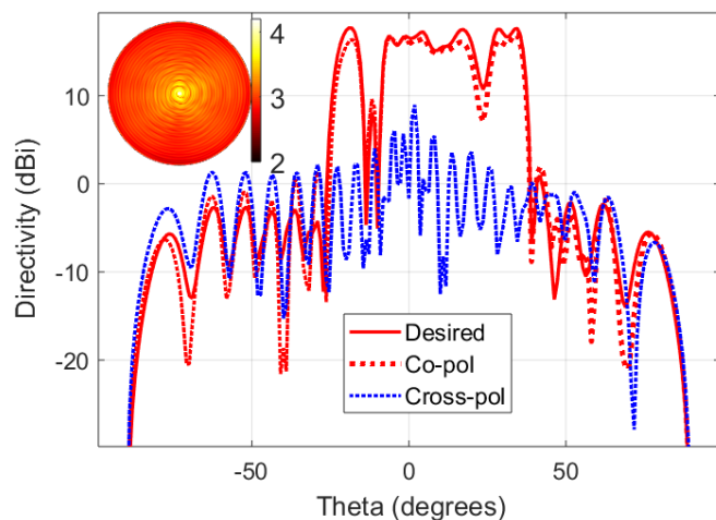
Fig. 3. Radiation pattern of the designed “fish-like” radiating MTS in the plane \alpha = 0 . The co-polar and the cross-polar pattern corresponds respectively to the Right Handed Circular Polarization (RHCP) and the Left Handed Circular Polarization (LHCP) directivity. The inset disk corresponds to the absolute value of the current distribution on the designed MTS (on \log_{10} scale) for a unit current excitation.
