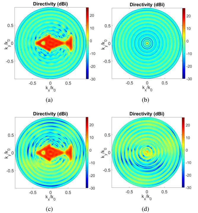
Fig. 2. Circularly polarized “fish like” radiation pattern in the (k_x, k_y) plane. (a): Co-polar component for the ideal antenna (desired pattern) (b): Cross-polar component for the ideal antenna (c): Co-polar component for designed MTS (d): Cross-polar component for designed MTS.
